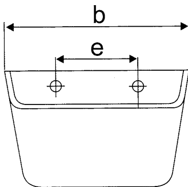
BE type plastic elevator buckets (parameters in mm)
